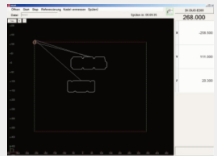
0002 Software DiSoft
